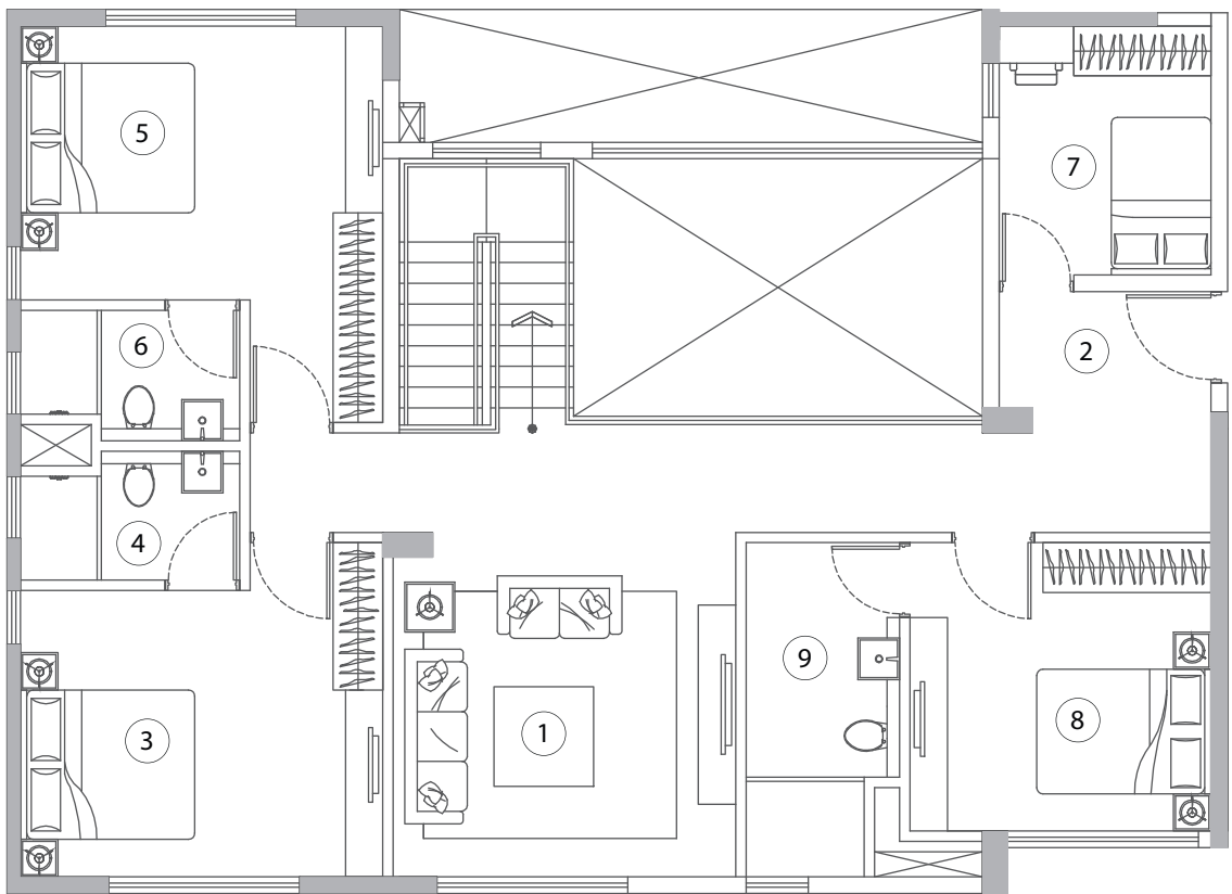
UNIT A DUPLEX UPPER (FLOOR - 11)
