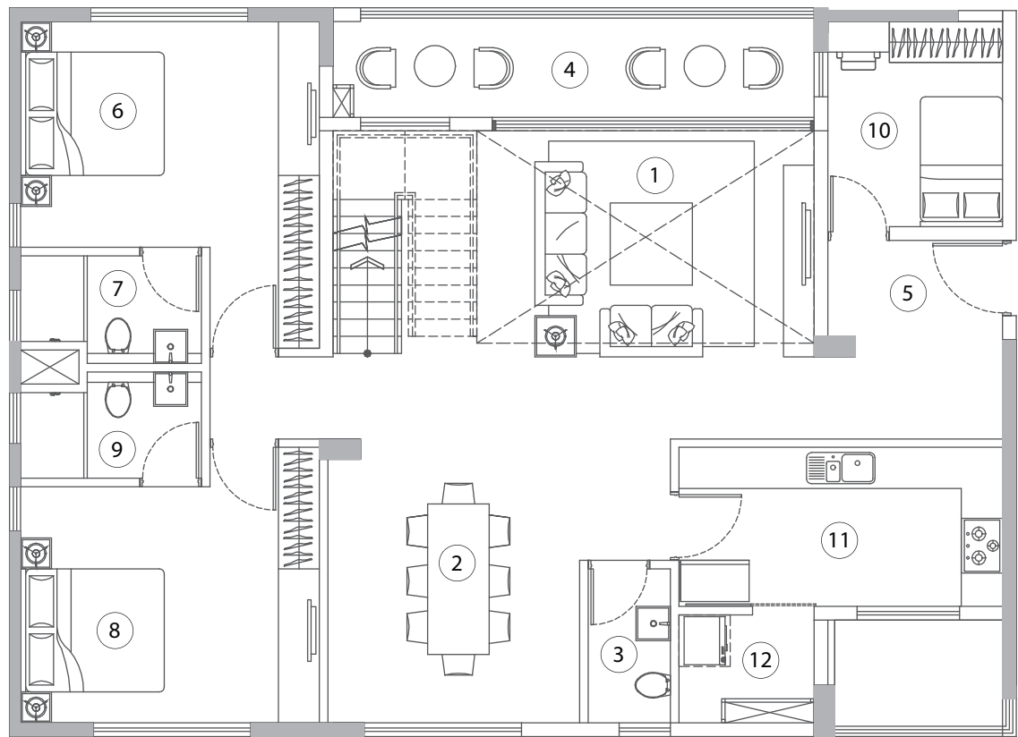
UNIT A DUPLEX LOWER (FLOOR - 10)
