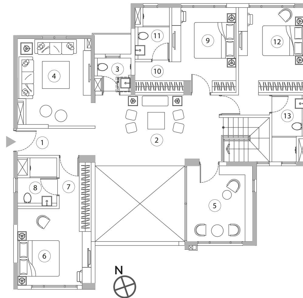
UNIT B DUPLEX UPPER (FLOOR - 2)
